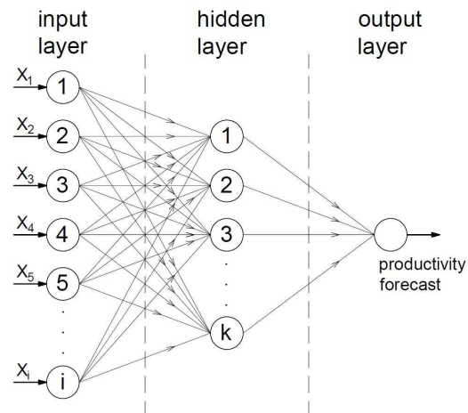
Figure 1: ANN model architecture
