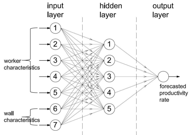
Figure 3. ANN model of bricklaying labour productivity
