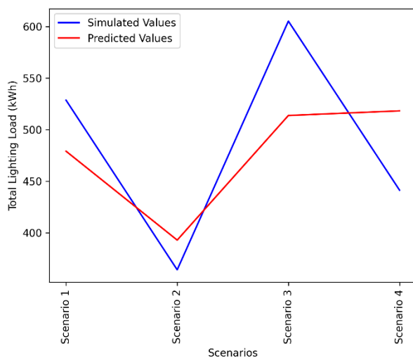
Figure 6: The total lighting energy load
