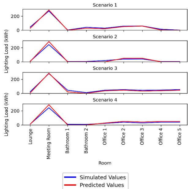
Figure 5: Total lighting energy load of different rooms
