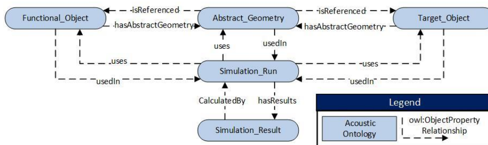
Figure 3: Representation of extension of the acoustic ontology.
