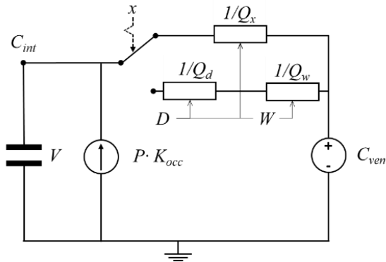
Figure 3: RC-network of the used model
