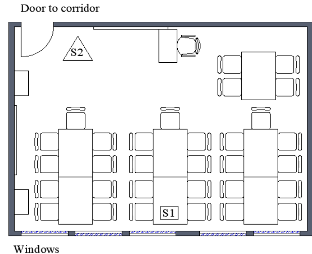
Figure 1: Layout of A1 (left) and A2 (right) classrooms and corresponding sensor location
