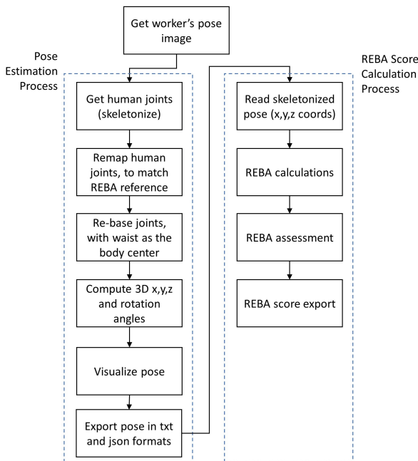
Figure 5: Human pose analysis flowchart.
