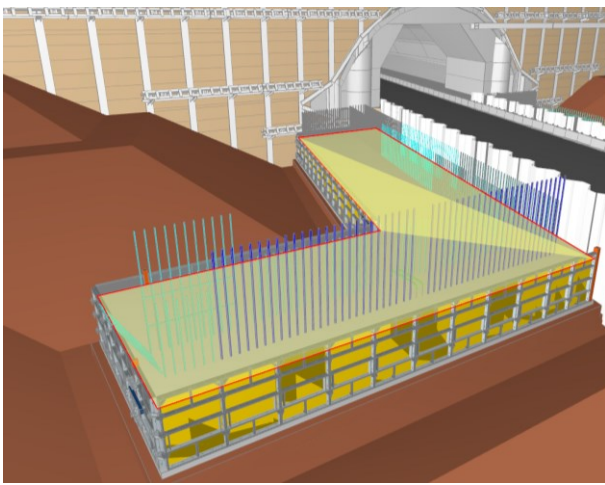
Figure 3: Simplification of the task “Construction of the foundation axis 10 (west), Pouring concrete”
