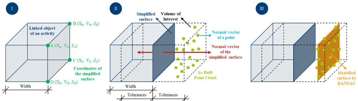
Figure 7: Surface-based progress track procedure
