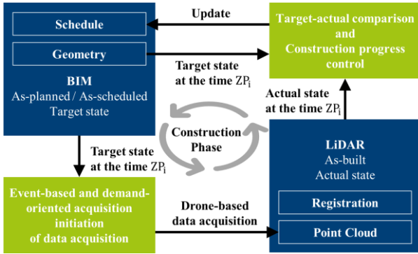
Figure 5: Construction progress control in project execution
