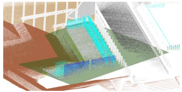
Figure 6: The identified surface of top edge concrete by RANSAC for the task "Construction of the foundation axis 10 (west), Pouring concrete"
