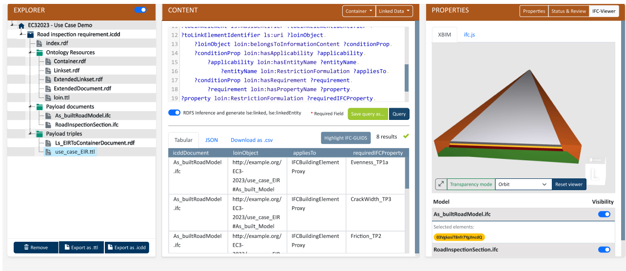
Figure 7: SPARQL query and results for container document specifications defined with LOIN ontology using the ICDD platform developed by Hagedorn et al. (2023)
