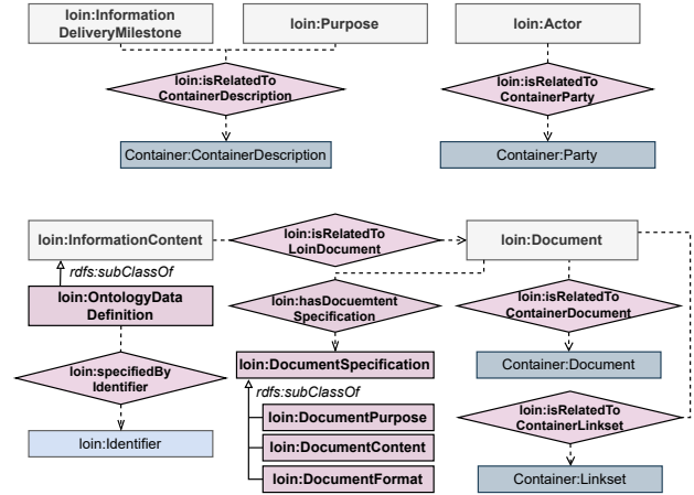
Figure 4: LOIN extension for referring to ICDD containers
