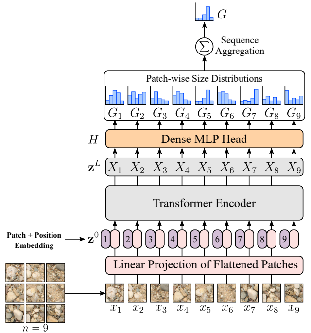
Figure 3: Overview on the proposed Granulometry Transformer architecture. A sequence of linearly projected and flattened image patches are fed to a transformer encoder and a MLP head is used on top of the architecture to predict a particle size distribution for each patch. The final grading curve for the image is calculated by aggregating the patch-wise distributions.
