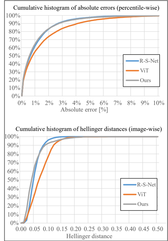
Figure 6: Cumulative histogram of absolute errors (top) and of the Hellinger distance (bottom) obtained on the D_{\text{coarse}} data set.
