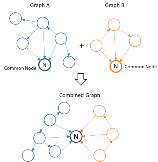
Figure 7: Example to show how the five component graphs are merged in Neo4j.
