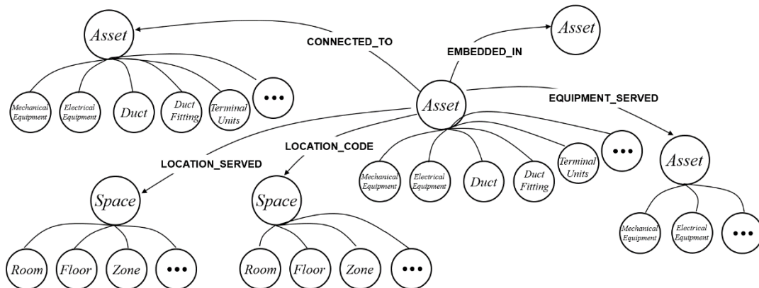
Figure 5: Graph Model Ontology.
