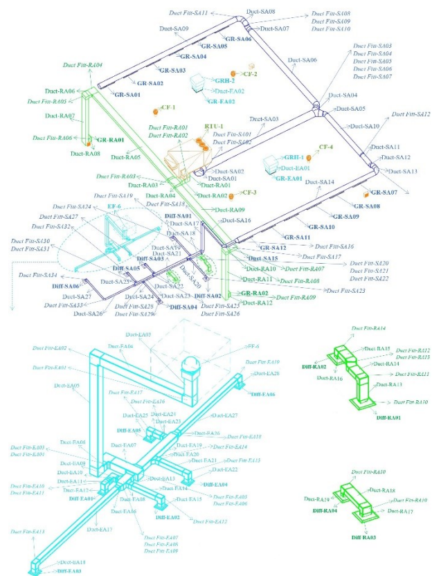
Figure 2: 3D Revit model of Zone 4 mechanical system showing components with their unique ID.
