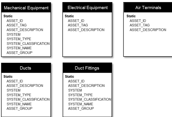
Figure 4: Data model for Zone 4 mechanical system.
