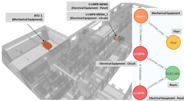
Figure 8: Highlighted components in the Navisworks model based on Neo4j scenario query.
