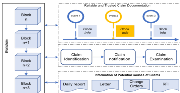
Figure 1: The proposed system architecture.
