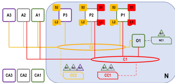
Figure 4: Designed Fabric network's configurations for a claim management system
