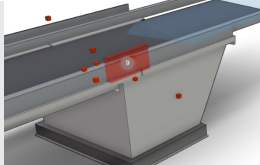
Figure 7: Comparison of the original damage documentation of SIB Bauwerke (left) and the created geometric representation and localisation in the IFC model (right). [Bold: location description terms, Italic: Free text field information]
