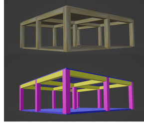
Figure 3: 3D model for training
