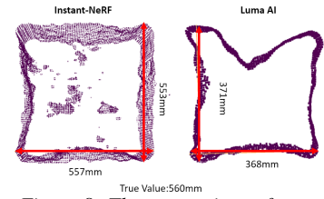
Figure 8: The comparison of accuracy on column size
