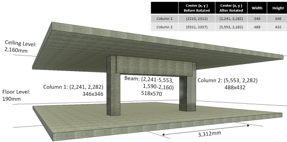
Figure 11: Execution to BIM
