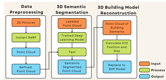
Figure 1: Framework of NeRF-to-BIM
