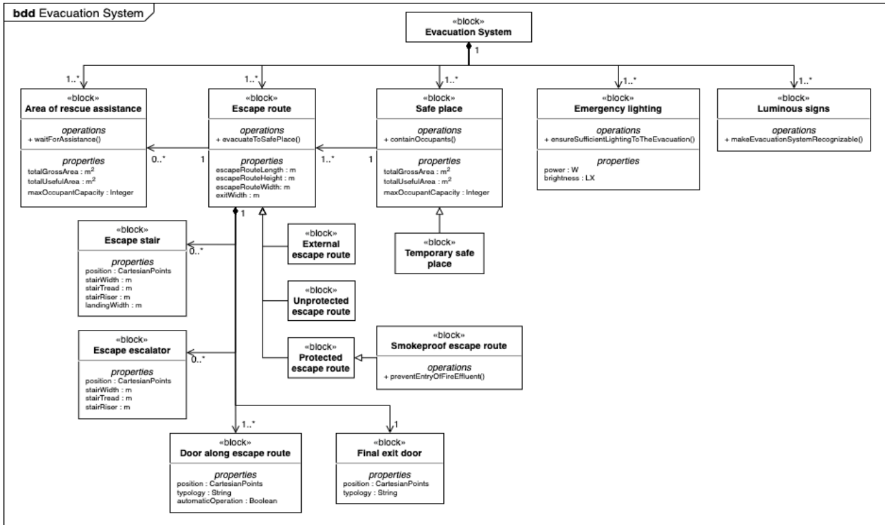
Figure 4: Evacuation Block Definition Diagram (ES02)
