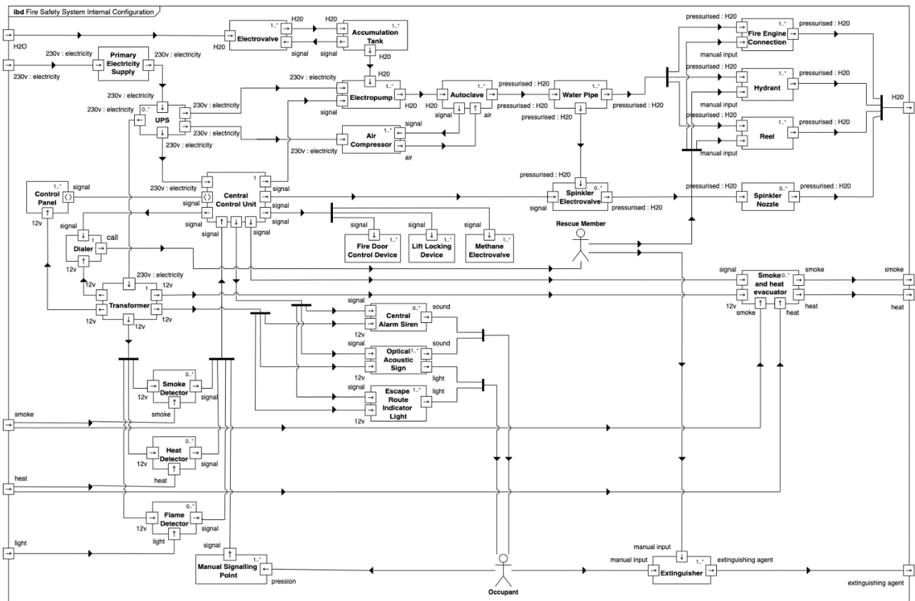
Figure 7: Fire Detection-Control-Extinguishing-System Internal Block Definition Diagram (S02)
