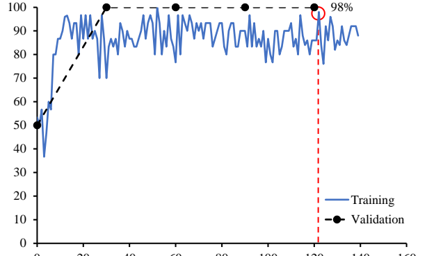
Figure 8: Training and validation accuracy history.
