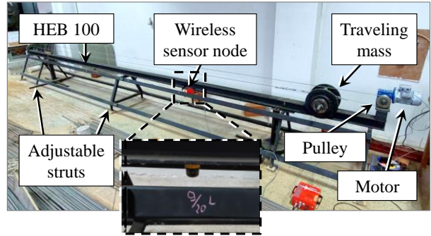
Figure 5: Experimental setup.
