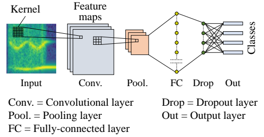
Figure 3: Layout of a typical CNN.
