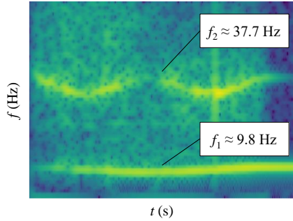
Figure 7: Gabor transform for the damaged beam ( m = 15 kg, |v| = 0.46 m/s).
